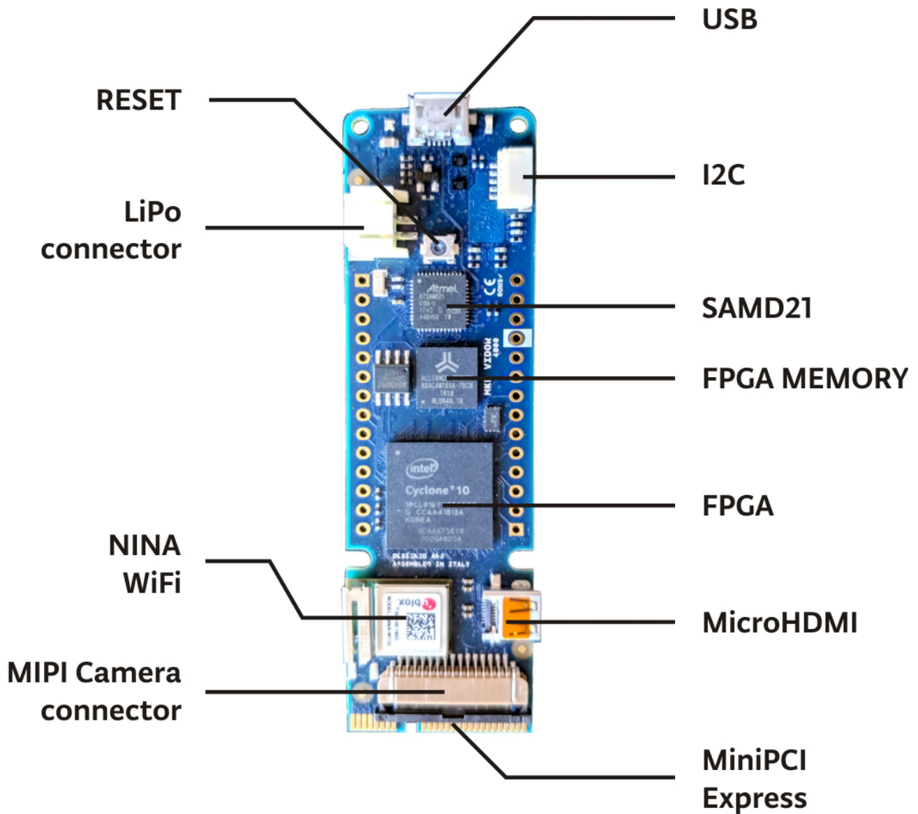
Board Overview
